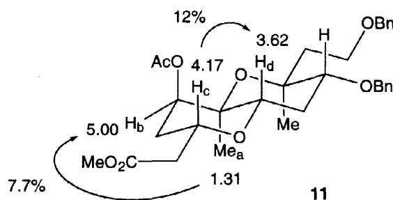
Figure 1. NOE experiments on the acetate 11 .
